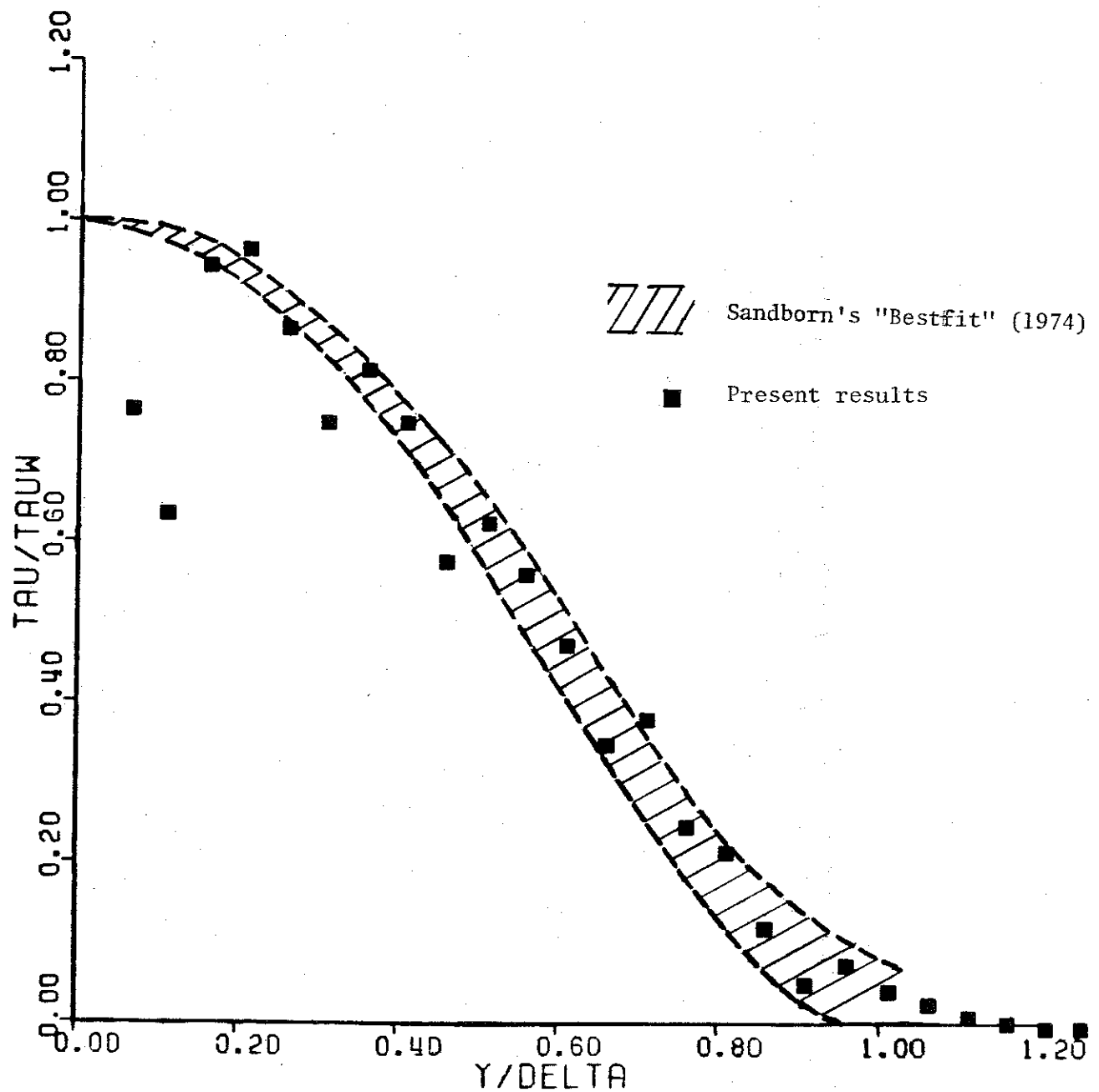
Fig. 2. Profiles of the Reynolds Shear Stress Normalized by the Surface Shear Stress, \tau/\tau_w ( \tau/\tau_w = -\bar{\rho} \overline{u'v'}/\rho_w u_\tau^2 ), at the Upstream Station ( X = -50.8\text{mm} ).
